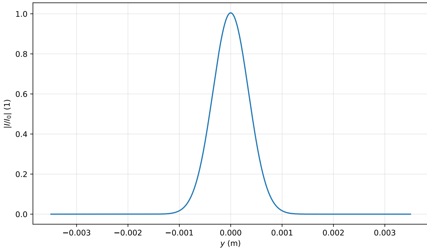
Intensity profile I(x=0, y, z=0.080)/I_0 , \text{Pin}=1.0\text{Pcr} , artificial time
